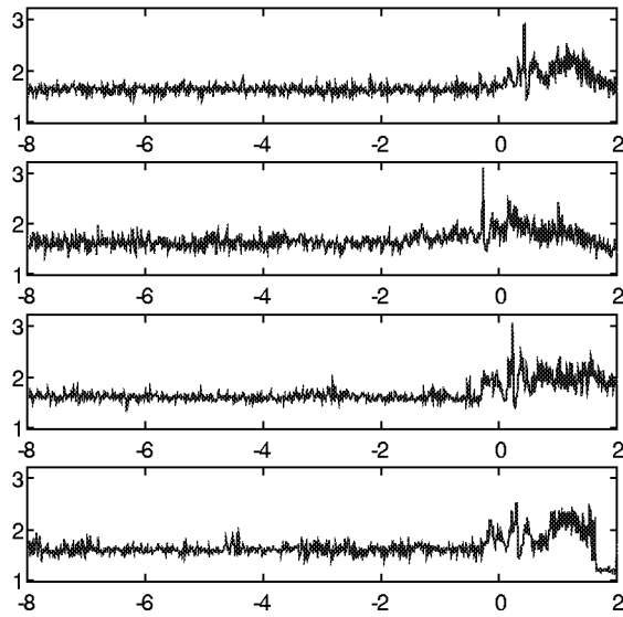
Figure 4: Fractal dimension over time (min) for patient 3, preictal (from -8 to 0 min) and ictal (from 0 to 2 min) periods
