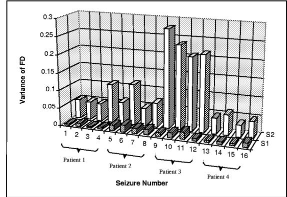
Figure 5: Variance of the fractal dimension for each record during preictal (S1) and ictal period (S2).
