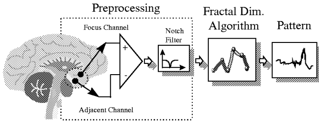
Figure 1: Methodology Diagram
