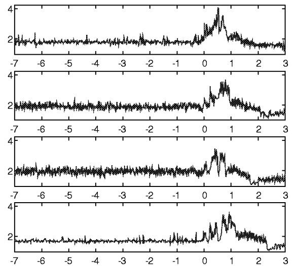
Figure 2: Fractal dimension over time (min) for patient 1, preictal (from -7 to 0 min) and ictal (from 0 to 3 min) periods.
