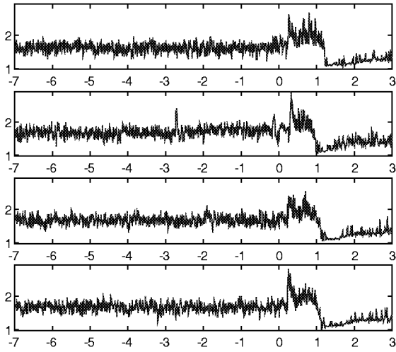
Figure 3: Fractal dimension over time (min) for patient 2, preictal (from -7 to 0 min) and ictal (from 0 to 3 min) periods
