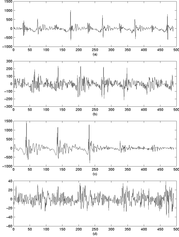
Figure 2: AR residuals for the impulsive model (3) for the voiced phonemes of Figure 1.
