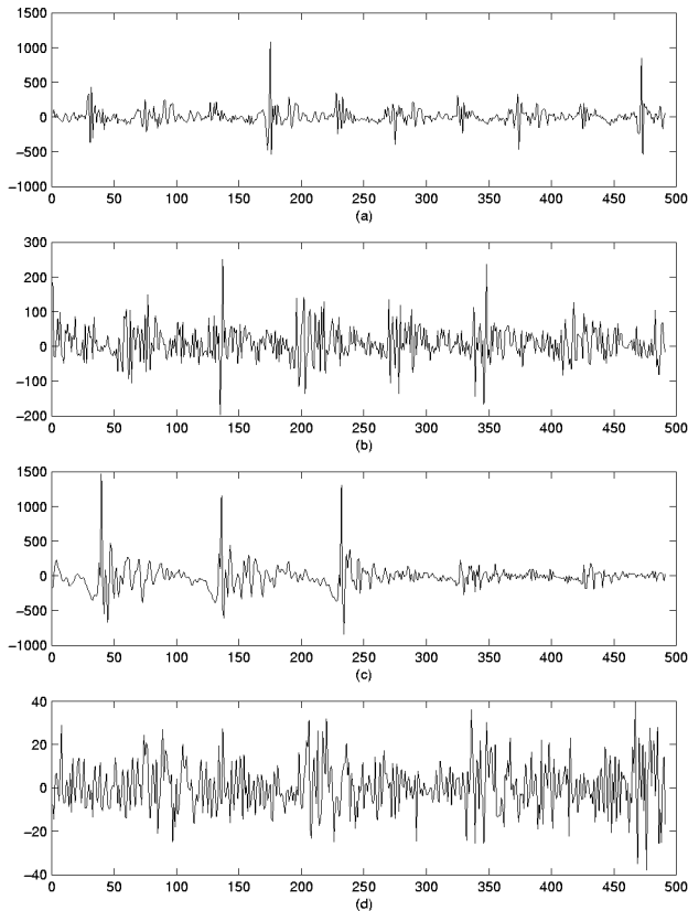
Figure 4: AR residuals for the LT model (12) for the voiced phonemes of Figures 1, 2.
