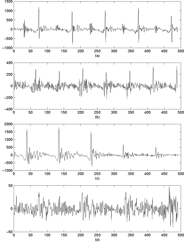
Figure 1: Plots of AR residuals for four voiced speech phones: (a) front /ae/, (b) diphthong /ay/, (c) semivowel /r/, (d) nasal /n/. The model (1) predicts that each of these signals be white (random) — clearly incorrect.
