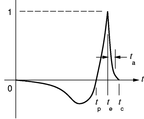
Figure 3: The LF deterministic excitation model.
