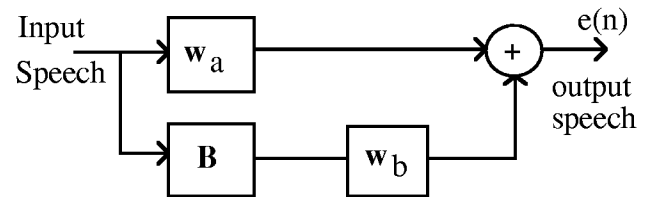
Figure 3. Generalized Sidelobe Canceller
