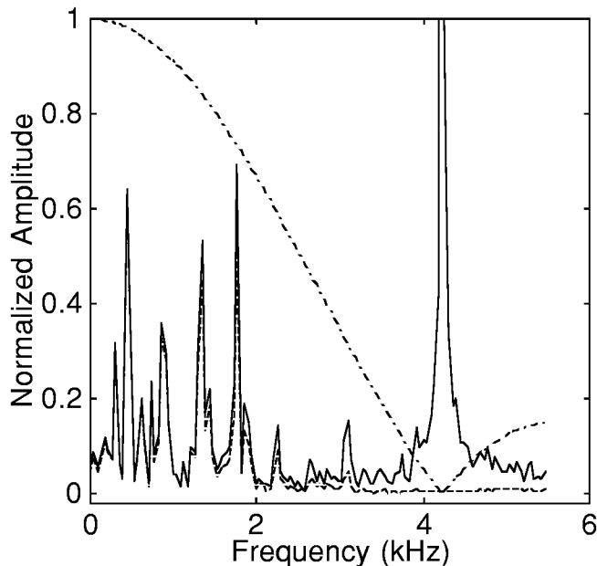
Fig. 2. Fourier Analysis and Notch Filtering (dash dot - filter frequency response, solid - normalized magnitude of DFT of original speech, dashed - normalized magnitude of DFT of filtered speech).
