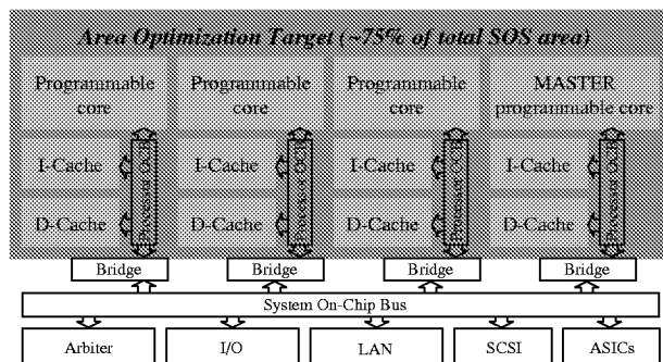
Figure 1: A typical multiprocessor SOS.
