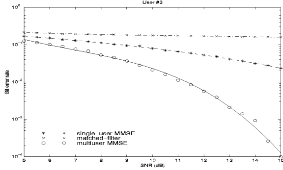
Figure 1. Comparison of bit error rate vs. signal-to-noise ratio (SNR) for three receivers: single-user space-time matched-filter, single-user space-time MMSE receiver and multiuser space-time MMSE receiver.
