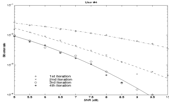
Figure 2. Bit error rate vs. SNR of the iterative interference cancellation method (first 4 iterations).
