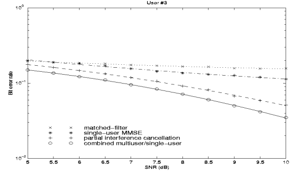
Figure 3. Bit error rate vs. SNR for four receivers in the presence of unknown interferers.
