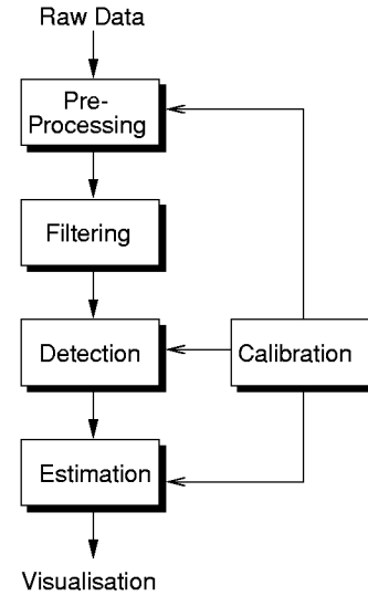
Figure 3: A block diagram showing processing applied to the raw radar data to provide coal depth estimates.
