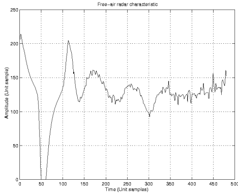
Figure 4: Typical radar–air coupling characteristic of the impulse radar directed into free space.
