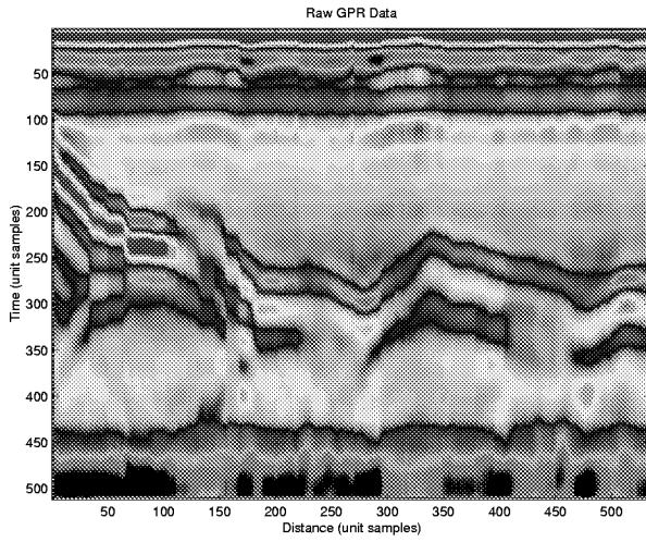
Figure 2: Raw GPR signals. The vertical axis is time delay, and the horizontal axis is distance.
