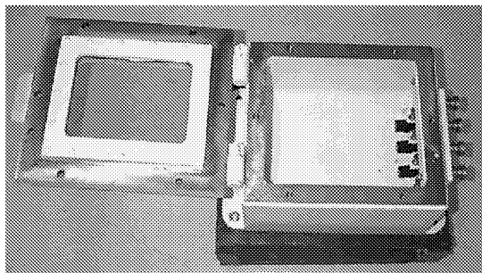
Figure 6: Flameproof enclosure which houses the signal processing and display components of the GPR system. The operator push-button controls are shown on the right.
