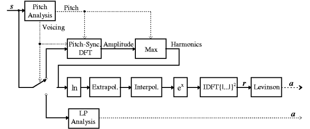
Figure 1. Block diagram of the voicing dependent frequency-domain spectral envelope estimation.
