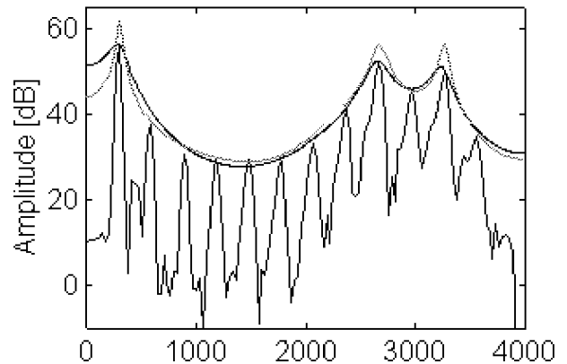
Figure 2. Spectral envelope modeling results. The estimation from harmonics is drawn in black line and the LP representation is drawn in gray line.
