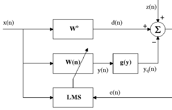
Figure 1. Block diagram of the system analyzed.
