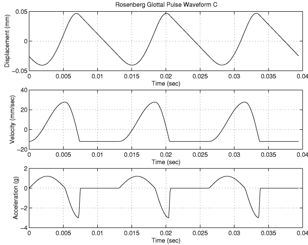
Figure 8. Displacement, velocity and acceleration curves for an EL excitation based upon the Rosenberg glottal pulse type C [3], scaled to 1 g rms acceleration. This excitation results in a very unnatural, metallic speech quality.
