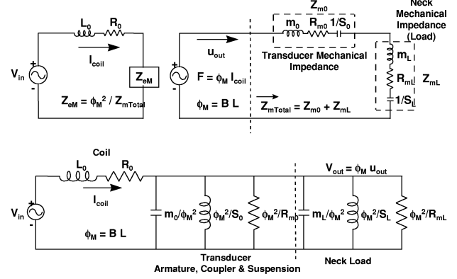
Figure 4. (top) Linear transducer electro-mechanical equivalent circuit diagram. The mechanical impedance of the neck serves as the load to the device. (bottom) Purely electrical equivalent circuit.
