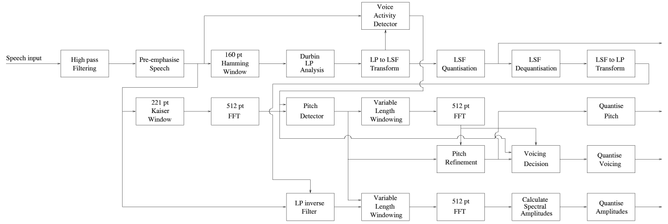
Figure 1: Block diagram of the Split-Band LPC encoder
