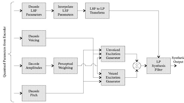
Figure 2: Block diagram of the Split-Band LPC decoder
