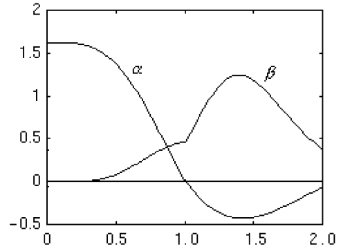
Figure 2. Values of \alpha and \beta that minimize MSE (Equation 2) for \hat{f}(u,v) = \text{sinc}^2(su,sv) .
