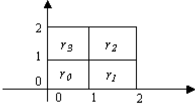
Figure 1. 2-D non-separable convolution kernel defined on [0,2] \times [0,2] . This can be generalized to [-2,2] \times [-2,2] by symmetry: r(x,-y)=r(x,y) and r(-x,y)=r(x,y) .
