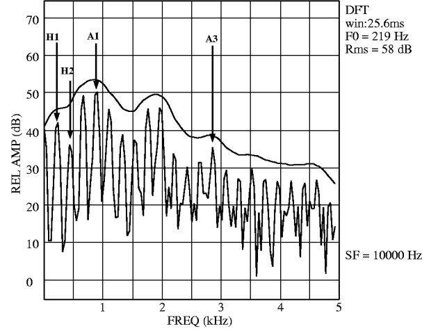
Figure 2: Example of the acoustic features associated with the speech spectrum of a vowel. The acoustic features are measured from the lower curve, which is the spectrum with a time window of 25.6 ms. The upper curve is a smoothed and offset version of the spectrum, and is not used to determine the amplitude of the labeled acoustic features.
