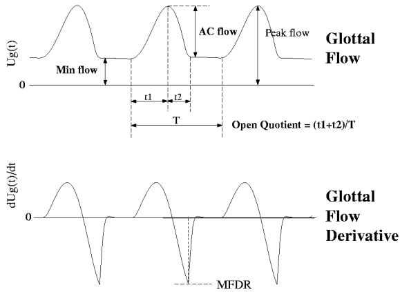
Figure 1: Definition of the aerodynamic features associated with the glottal flow waveform U_g(t) and the flow derivative waveform dU_g/dt . The Maximum Flow Declination Rate (MFDR) is indicated on the flow derivative waveform.
