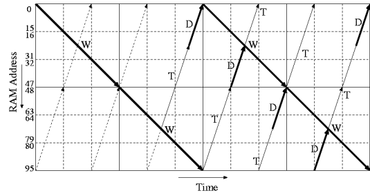
Figure 5: Trace Back Operation
