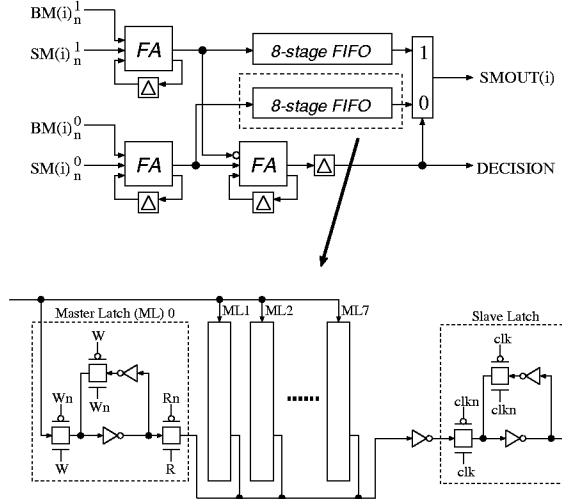
Figure 3: Bit-serial ACS unit
