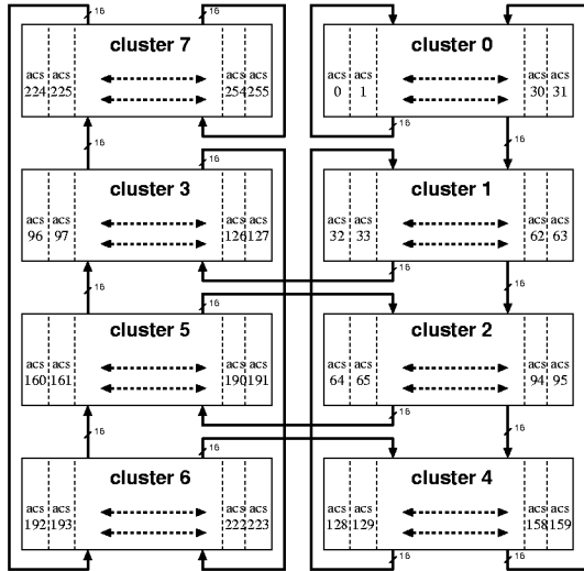
Figure 4: Floor plan of the ACS module.
