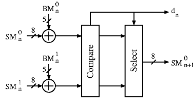
Figure 2: ACS unit diagram
