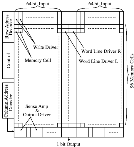
Figure 6: 128×96 Survivor Path Memory
