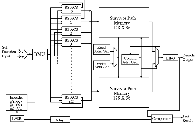
Figure 1: Bit-Serial Viterbi Decoder Chip Diagram
