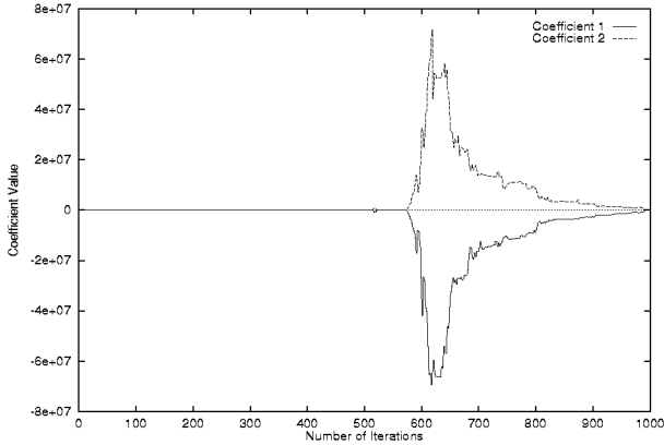
Figure 2: Trajectory of w_{1,k} and w_{2,k} for \mu = 0.5
