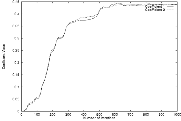
Figure 1: Trajectory of w_{1,k} and w_{2,k} for \mu = 0.005
