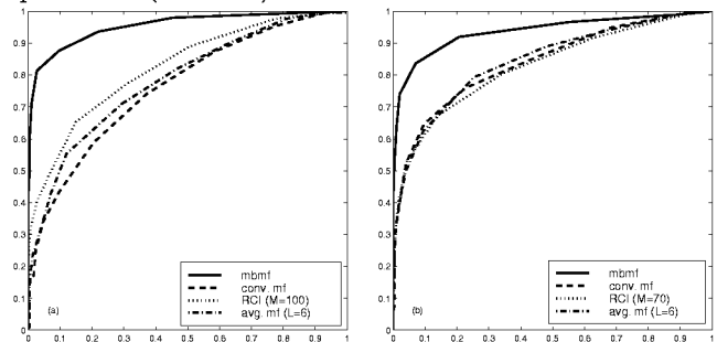
Figure 3: ROC curves for ranges of (a) 1.19 km and (b) 0.6 km obtained with the optimal model-based matched-filter, the conventional source-receiver matched-filter, the RCI processor, and the new ad-hoc detector.
