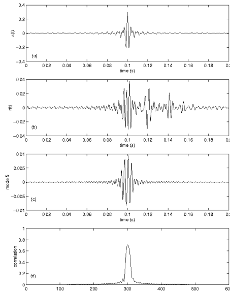
Figure 1: (a) Transmitted sequence. (b) Received sequence. (c) Mode 5 of the received sequence. (d) Correlation between the transmitted sequence and mode 5.
