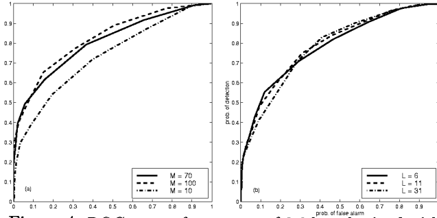
Figure 4: ROC curves for a range of 0.6 km obtained with (a) the RCI processor for different values of M , and (b) the new ad-hoc processor for different values of L .
