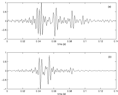
Figure 2: Impulse ocean response for a receiver at a depth of 94.125 m and a source at a depth of 64 m and range of (a) 1.19 km and (b) 0.6 km.
