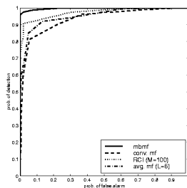
Figure 5: ROC curves for SWelEX data.
