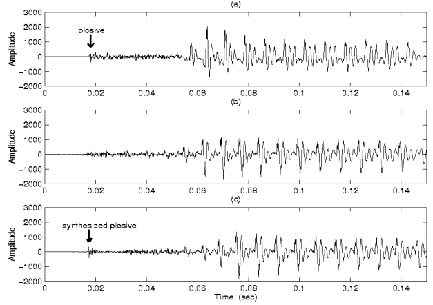
Figure 2: Reproduction of the plosive signal in the synthesized speech. (a) Input speech signal. (b) Synthesized speech signal by the Federal Standard MELP. (c) Synthesized speech signal by the improved MELP.
