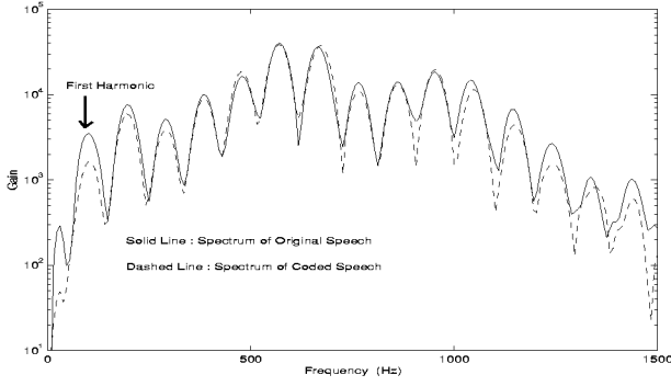
Figure 4: Fourier magnitudes of speech for a low-pitch male speaker. A solid line and a dashed line are the spectrum of the original and the coded speech respectively.
