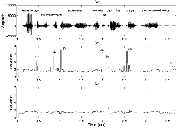
Figure 3: Plosive signal detection. (a) Input speech signal. (b) Peakiness value with sliding window. (c) Peakiness value with fixed position window.
