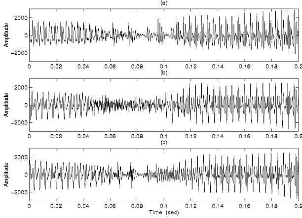
Figure 1: Elimination of the artificial noise at the junction of two vowel segments. (a) Input speech signal. (b) Synthesized speech signal by the Federal Standard MELP. (c) Synthesized speech signal by the improved MELP.
