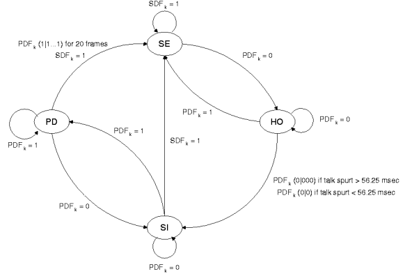
Figure 2: State transition diagram of the decision box. SI stands for silence state. PD stands for primary detection state. SE stands for speech detected frames. HO stands for hangover state.
