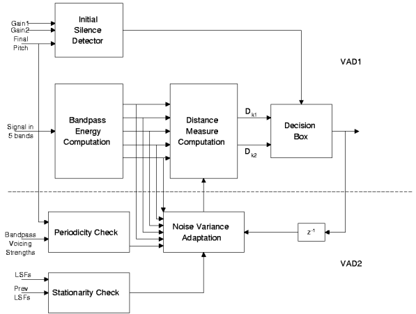
Figure 1: Voice Activity Detector for VBR-MELP Vocoder.
