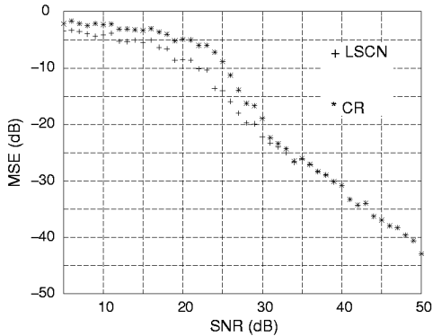
Figure 3: Comparison between LSCN and CR methods for the ill-conditioned channel case ( \delta = \pi/10 ).
