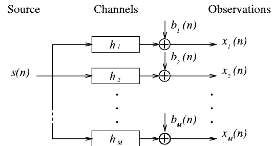
Figure 1: Multi-channel FIR system.
