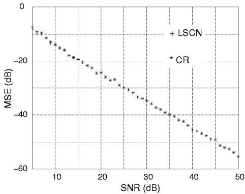
Figure 2: Comparison between LSCN and CR methods for the well-conditioned channel case ( \delta = \pi ).
