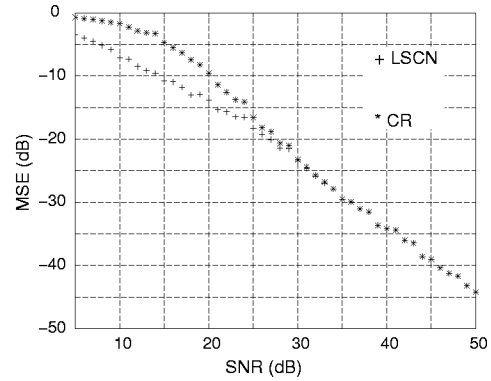
Figure 4: Comparison between LSCN and CR for three random channels.
