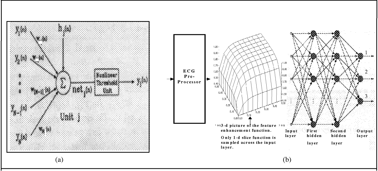
Figure 3: Architecture of the 4-layer neural network. (a) Neuron or processing unit in the network. (b) The four-layer neural network. Only 1-d slice of the weight function modifies the corresponding cumulant slice.
