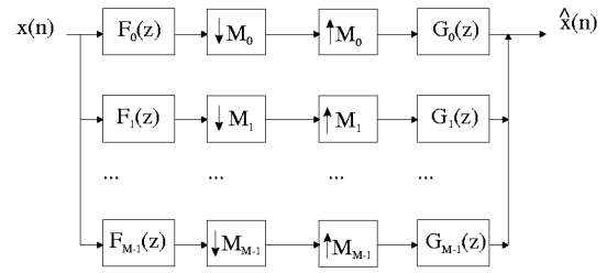
Figure 1: Uniform M -channel analysis/synthesis banks.
