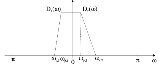
Figure 2: Desired frequency response D(\omega) .
