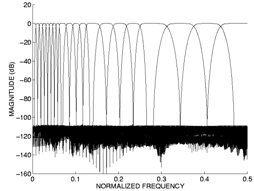
Figure 4: Analysis filters frequency responses relative to a nonuniform 20-channel bank. The prototype is designed by using recursively updated weighting functions.
