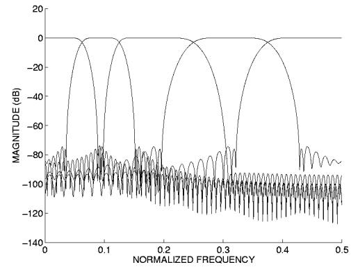
Figure 3: Analysis filter frequency responses relative to a nonuniform 5-channel bank. The prototypes are designed by using the eigenfilter method to approximate the ideal frequency responses defined in either (10) or (12).
