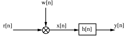
Figure 3: Diagram of model used to determine the effect of using a subsequence of input sample stream to compute channel filter output.
