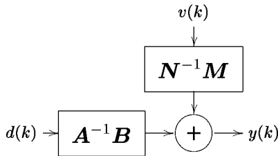
Figure 1: The multivariable system model.
