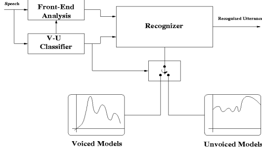
Figure 1: Block diagram of the V-U-based CSR system illustrating how the V-U decision affects both pre-processing and post-processing stages.
