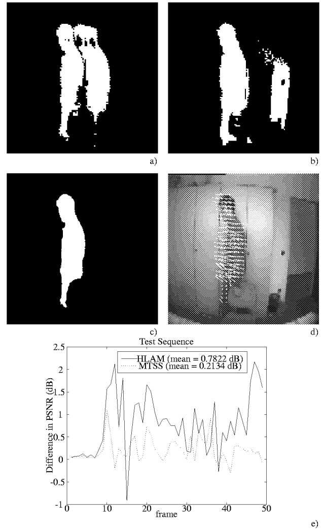
Figure 3: Simulation results (frame #19): Extracted foreground using a) the RTL-filter method ( \alpha = 0.5 , \lambda = 20 ), b) the Kalman method ( \lambda = 20 ), and c) the ARTL-filter method ( g_B = 0.001 , t_{min} = 10 , t_{max} = 40 , o = 6 ). d) Original frame with superimposed motion vector field. e) Performance comparison in terms of the difference in PSNR with respect to the ES technique.
