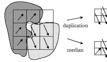
Figure 2: Down conversion of the central block using duplication and median of the neighborhood.
