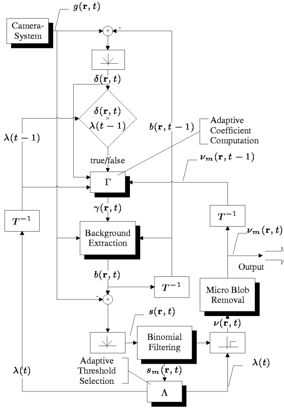
Figure 1: Flowchart of the ARTL-filter method.
