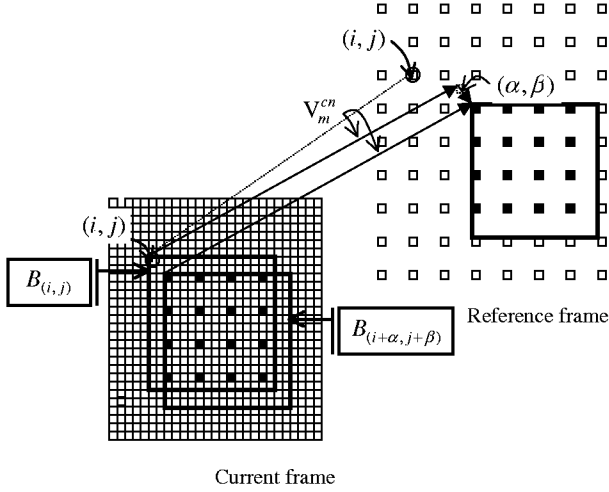
Figure 4. A V_m^{cn} search at level 0 in case of L=3 . Black colored pixels are to be matched each other in SAD
