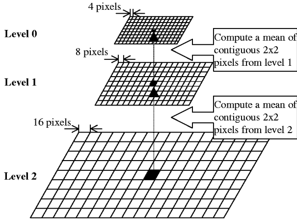
Figure 1. Multi-resolution frame structure for the reference frame ( L=3 ). Each rectangle denotes a macroblock (MB).
