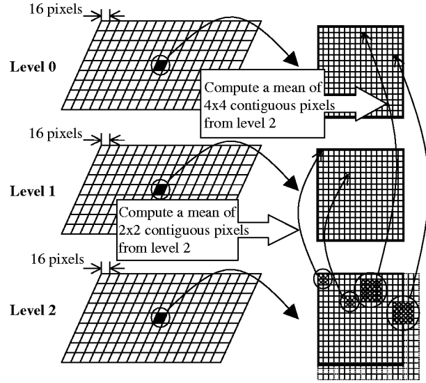
Figure 2. Block mean pyramid frame structure for the current frame ( L=3 ). Each rectangle denotes a MB.
