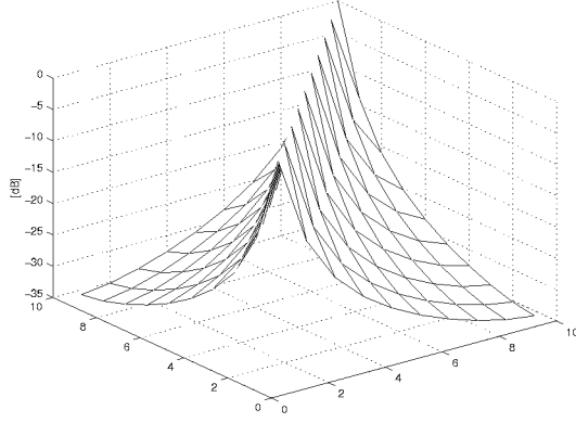
Figure 2: The magnitude of the elements of the coupling matrix of an array of 10 \lambda/2 dipoles spaced \lambda/2 apart.
