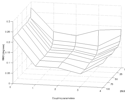
Figure 3: The RMS error for \phi = 80^\circ when jointly estimating DOA and coupling using the array in Figure 2 when two waves are incident from (80^\circ, 85^\circ) and 1000 snapshots.
