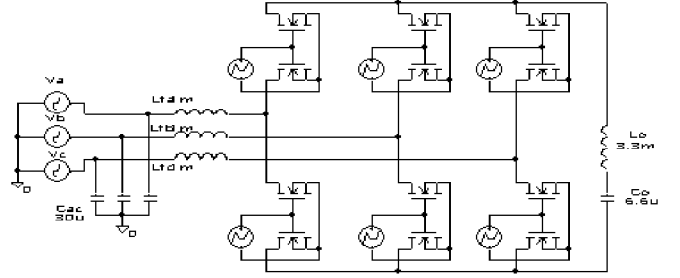
Figure 3. The active filter circuit diagram in PSpice.
