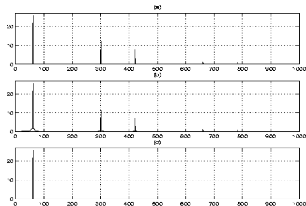
Figure 6. The Matlab simulation results (a) FFT of nonlinear load current (TDD = 57%) (b) FFT of the generated active filter current (c) the FFT of conditioned ac line current (TDD \approx 0%).
