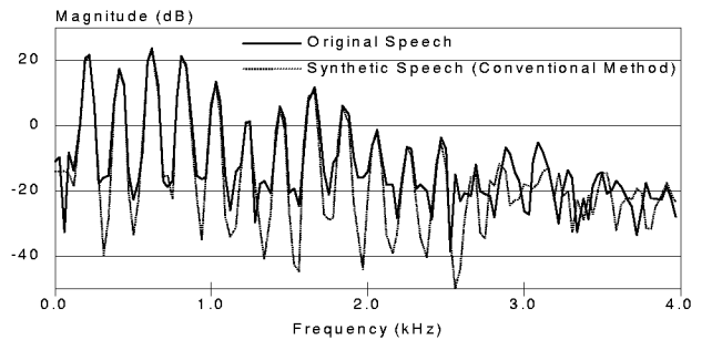
Figure 3(a) A typical speech spectrum (solid curve) and the corresponding synthetic spectrum (dotted curve) obtained using conventional V/UV mixing model.
