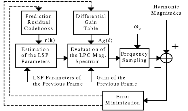
Figure 1 A block diagram of the proposed closed-loop quantization technique.
