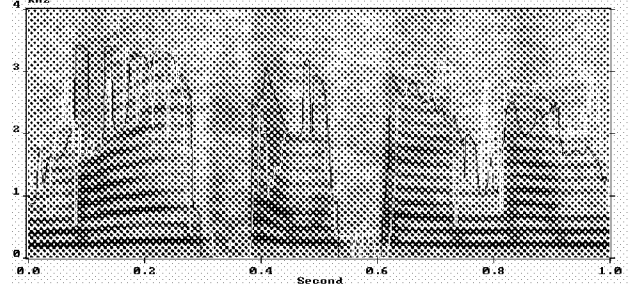
Figure 2 Speech spectrogram and its V/UV transition curves obtained from closed-loop analysis (white curve) and proposed method (dark curve).
