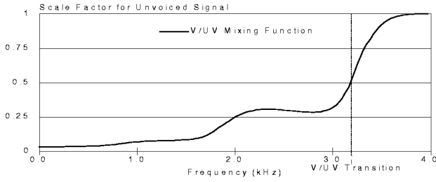
Figure 3(b) The V/UV mixing function v(\omega) derived from speech spectrum shown in Fig. 3(a).
