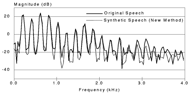
Figure 3(d) A typical speech spectrum (solid curve) and the corresponding synthetic spectrum (dotted curve) obtained using the improved V/UV mixing model.
