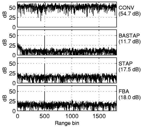
Figure 4: Filter outputs with OINR.
