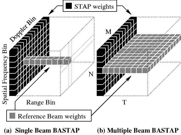
Figure 3: Beamspace interpretation of BASTAP.
