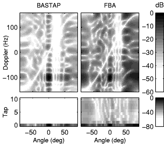
Figure 6: 2D Beampatterns.
