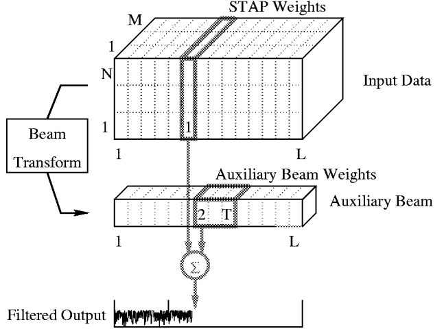
Figure 2: Beam Augmented STAP architecture.
