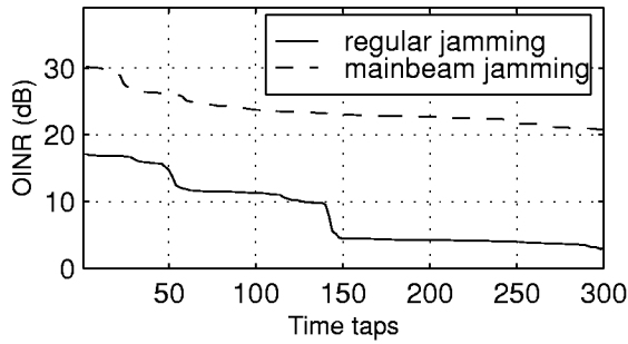
Figure 5: OINR vs. number of taps.
