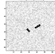
Figure 8: The 26th image of the orbiting and translational motion image sequences .
