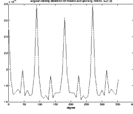
Figure 4: The angular velocity \theta_1 corresponding to \vec{v}^* = (1, 0) for the image sequences. The unit of the x-axis is degree. The eight peaks correspond to n * \pi/4 (i.e. 45^\circ n ) within [0, 2\pi) , n=0, 1, \dots, 7 .
