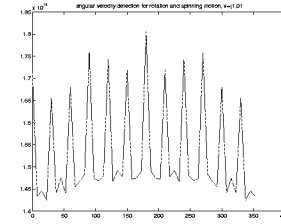
Figure 11: The angular velocity \theta_1 corresponding to \vec{v}^* = (1, 1) , The unit of the x-axis is degree. The twelve peaks correspond to \pi/6 * n (i.e. 30^\circ n ) within [0, 2\pi) , n=0, 1, \dots, 11 .
