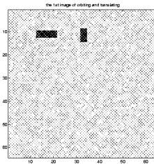
Figure 7: The first image from the image sequences with two objects undergoing orbiting and translating motion. One has initial orbiting center at (16,33), its translational velocity \vec{v}^* = (1, 0) , and its angular velocity \theta_1^* = \pi/4 . The other's initial orbiting center is at (10,10), its \vec{v}^* = (1, 1) and its \theta_1^* = \pi/6 . Noise is added.
