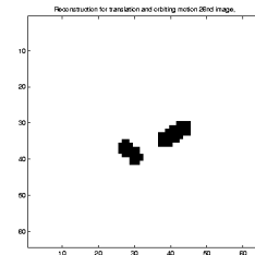
Figure 12: The reconstructed 26th image for orbiting and translating motion from the image sequences.
