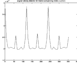
Figure 5: The angular velocity \theta_1 corresponding to \vec{v}^* = (0, 1) for the image sequences. The unit of the x-axis is degree. The six peaks correspond to n * \pi/3 (i.e. 60^\circ n ) within [0, 2\pi) , n=0, 1, \dots, 5 .
