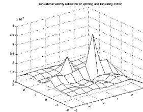
Figure 3: The translational velocity estimation, the two peaks correspond to \vec{v}^* = (1, 0) and \vec{v}^* = (0, 1)
