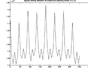
Figure 10: The angular velocity \theta_1 corresponding to \vec{v}^* = (1, 0) , The unit of the x-axis is degree. The eight peaks correspond to \pi/4 * n (i.e. 45^\circ n ) within [0, 2\pi) , n=0, 1, \dots, 7 .
