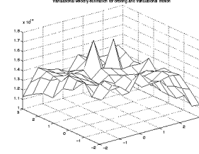
Figure 9: The translational velocity estimation. The two peaks correspond to \vec{v}^* = (1, 1) and \vec{v}^* = (1, 0)
