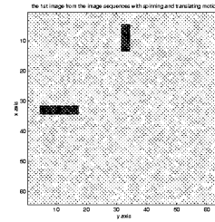
Figure 1: The first image from image sequences with two objects undergoing spinning and translating motion. One object with initial spinning axis at (8, 33) its translational velocity \vec{v}^* = (1, 0) and angular velocity \theta_1^* = \pi/4 , the other's initial spinning axis is at (33, 10) , it has \vec{v}^* = (0, 1) and \theta_1^* = \pi/3 . Noise is added.
