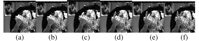
Figure 4. The image sequence tracking of two-digit gesture "12". The model transition does not be return to m_0 and the middle finger is straightened directly which can be described by m_2 . (a) shows the initial hand shape located near the real hand in the first frame, (b)~(f) present the state transition from model m_0 to model m_1 , then transition to model m_2 .
