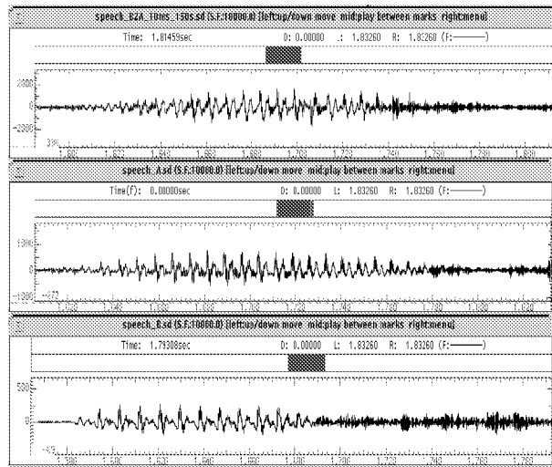
Figure 4: Waveform displays of “greasy” from “She had your dark suit in greasy wash water all year.” for modified northern (top), having the glottal flow and time-alignment of the original southern (center). The original northern (bottom) is also shown.
