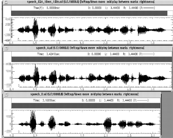
Figure 2: Waveforms displays of the utterance “She had your dark suit in greasy wash water all year.” for modified northern (top), having the glottal flow and time-alignment of the original southern (center). The original northern (bottom) is also shown.
