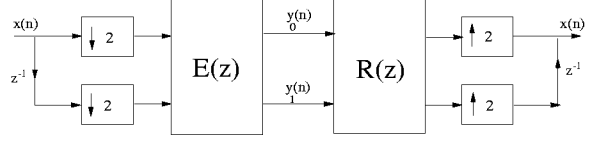
Figure 2: Polyphase representation of two band filter bank.
