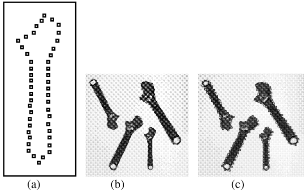
Figure 4. Detecting multiple objects with different scale, orientation, and local deformation. (a) Template. (b) Input image. (c) Detected objects.
