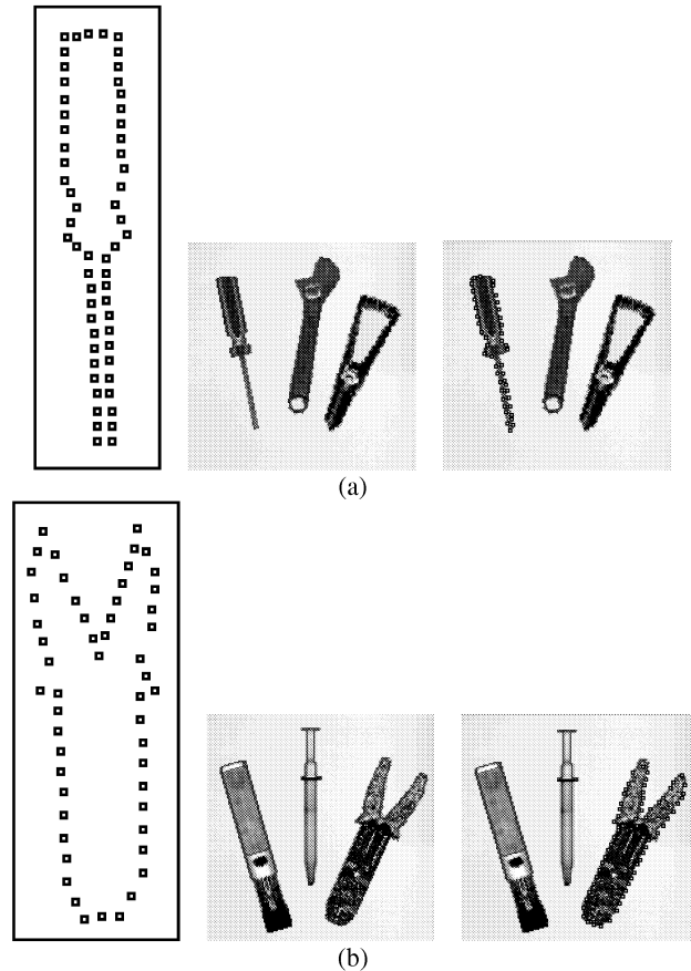
Figure 3. Automatic localization of desired objects. (a) Retrieval of a screwdriver using multiresolution deformable template matching. (b) Retrieval of a wire cutter using multiresolution deformable template matching. (From left to right: template, input image, retrieved deformed template.)
