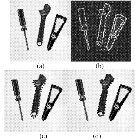
Figure 2. Object localization using multiscale. (a) Image at coarse scale. (b) Edge magnitude with initial contour. (c) Intermediate result at fine scale. (d) Final result.
