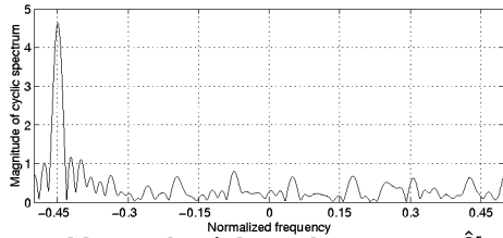
Fig. 3: Magnitude of the cyclic spectrum \hat{S}[1, f] .
