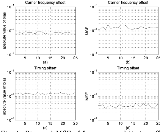
Fig. 1: Bias and MSE of frequency and timing offset estimators (13) and (14), respectively, versus SNR/dB: a) bias and b) MSE of \hat{\theta}_e , c) bias and d) MSE of \hat{n}_e/M .
