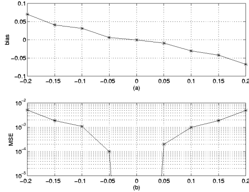
Fig. 2: (a) Bias and (b) MSE 9 of \hat{\theta}_e according to (13) versus \theta_e as a function of \theta_e .
