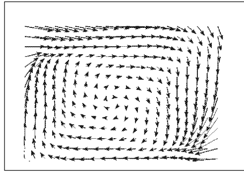
Figure 4: Computation of the interpolating vector field using the initial data of figure 3. Parameter \alpha = 0.1 .
