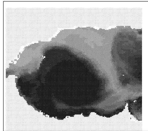
Figure 1: NOAA-AVHRR Sea Surface Temperature over the Alboran Sea. Image acquired on 24 august 1996. False colors.
