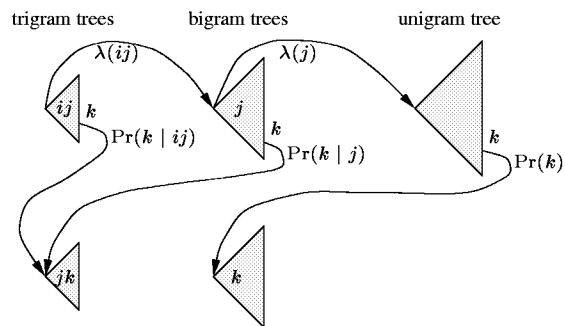
Figure 1: Partial view of the representation of the integrated network corresponding to the smoothed trigram model. \lambda(ij) and \lambda(j) are the interpolation parameters [1] (in practice, these values are the back-off normalizing factors).
