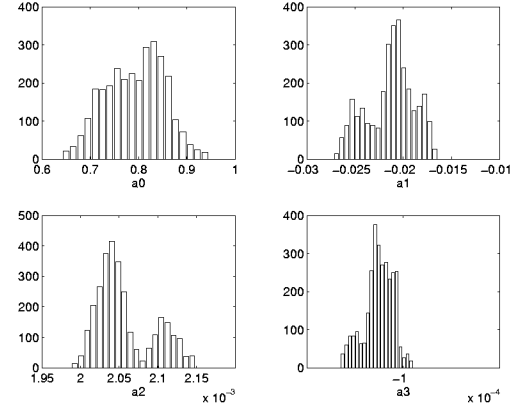
Figure 5: Estimation of the posterior distribution p(a_i|\mathbf{y}) , M = 4 , for 10dB
