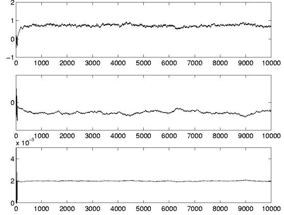
Figure 1: Generated chains for a_0 , a_1 and a_2 , rsb = 10dB (top to bottom)
