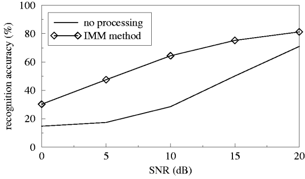
Figure 1: Recognition performance with additive white noise.
