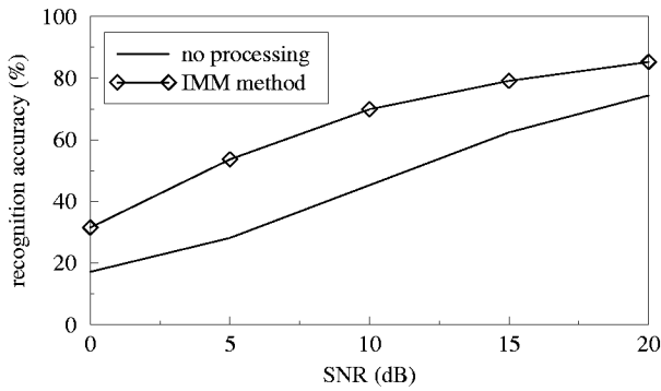
Figure 2: Recognition performance with additive babble noise.
