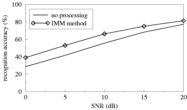
Figure 3: Recognition performance with additive impulsive noise.
