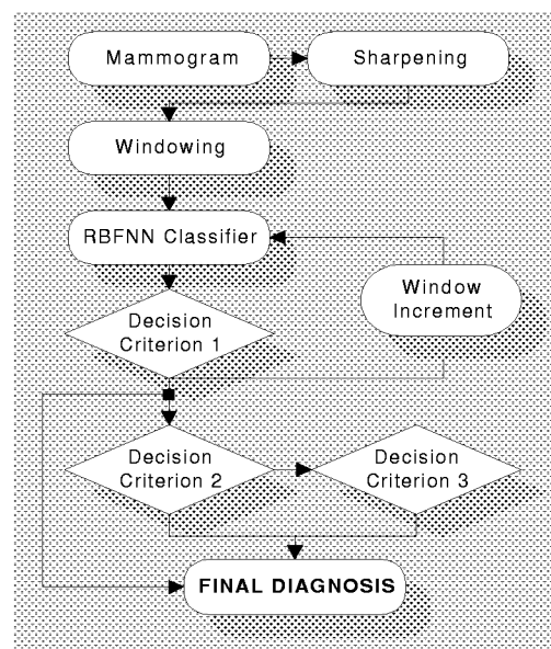
Figure 1. Structure of the proposed detector of circumscribed masses
