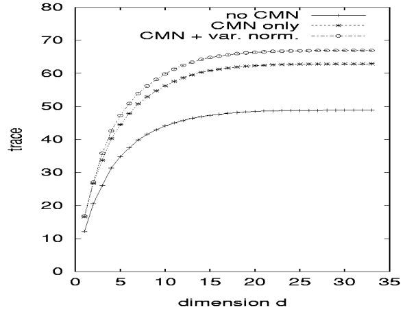
Figure 1: Trace criterion versus vector dimension on WSJ0 database (42 male and 42 female speakers) showing the effect of cepstral mean and variance normalization.
