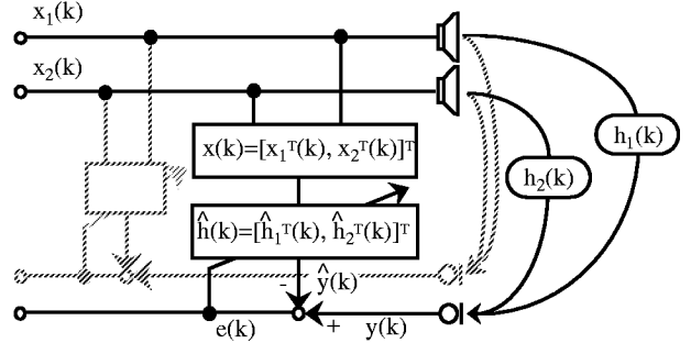
Figure 1: Configuration of stereo echo canceller.
