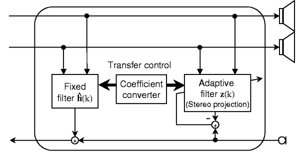
Figure 3: Stereo Duo-filter structure.
