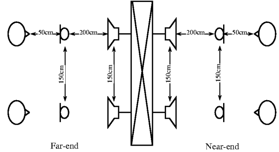
Figure 4: Positions of loudspeakers, microphones, and talkers.
