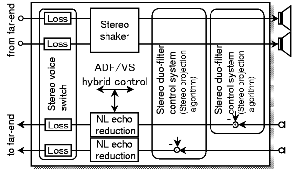
Figure 2: Developed stereo echo canceller.
