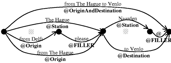
Figure 3. Corresponding concept graph.
