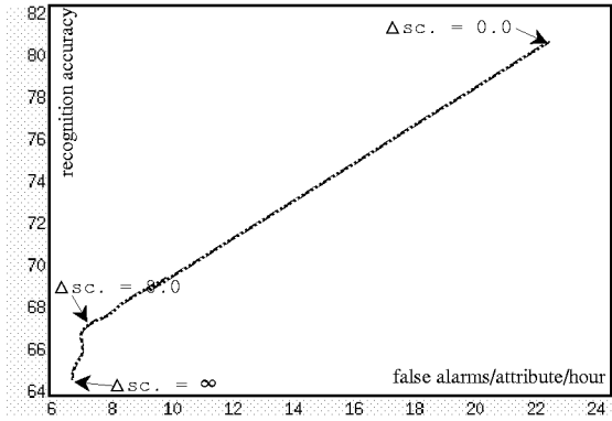
Figure 4. Receiver Operation Characteristic (ROC) curve.
