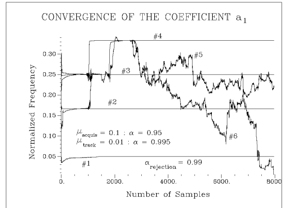
Figure 4-5: Coefficients of the PIRANHA Filter.
