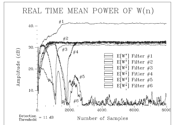
Figure 4-6: Signal w(n) for Cells Activation/Desactivation.
