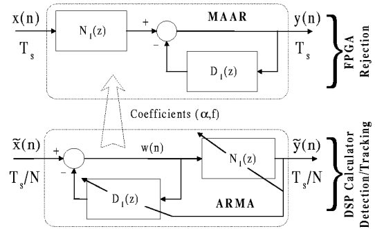
Figure 2-3: Main Structure of the PIRANHA Cell H_1(z) .
