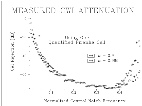
Figure 4-3: Measured CW Interference Attenuation (dB).
