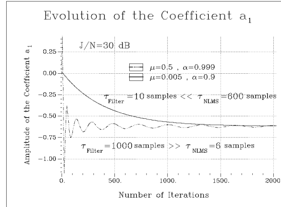
Figure 3-2 Transition Mode of the Adaptation.
