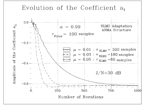
Figure 3-1 Convergence of NLMS Adaptation.
