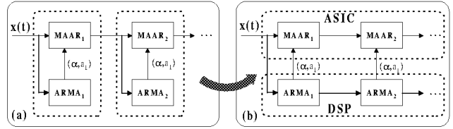
Figure 2-2: From Conventional to PIRANHA Structure.
