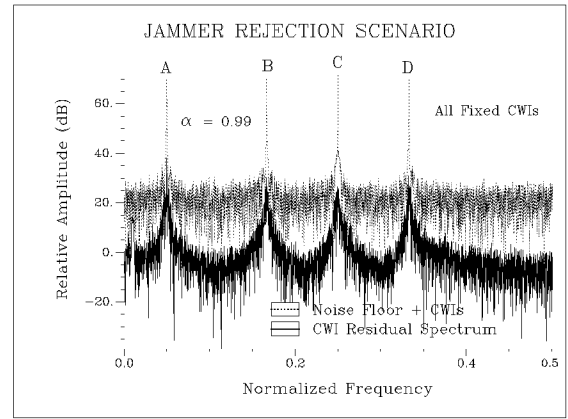
Figure 4-4: Vue of the Input and Residual Signal Spectrum.
