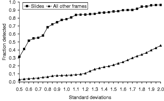
Figure 2. Slide detection performance vs. threshold.
