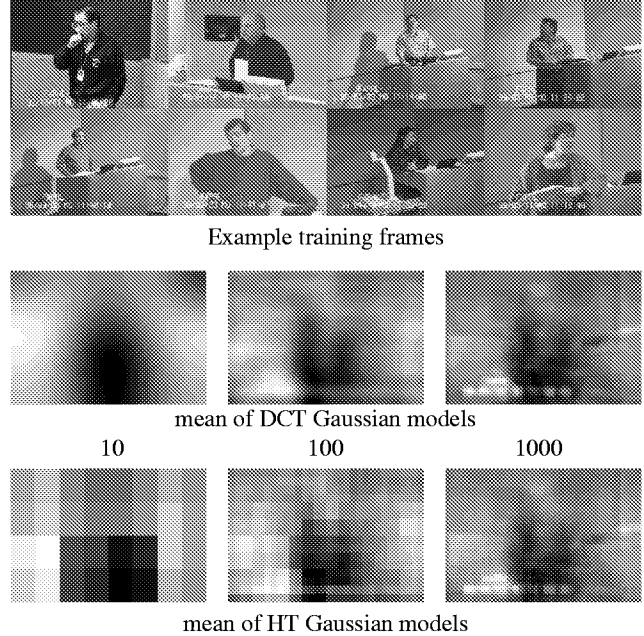
Figure 1. Example training frames and model means.
