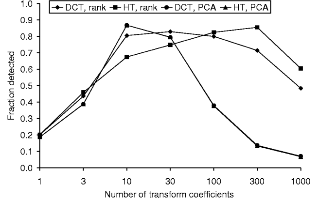
Figure 3. Classification vs. number of coefficients.
