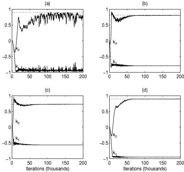
Figure 1: Trajectories of the reflection coefficients of the adaptive filter. (a) M = 1, C(z) = 1 , (b) M = 2, C(z) = 1 , (c) M = 3, C(z) = 1 , and (d) M = 1, C(z) = 1 + 0.0974z^{-1} - 0.9025z^{-2} . The stepsizes for the recursive and non-recursive part were 10^{-6} and 10^{-5} respectively.
