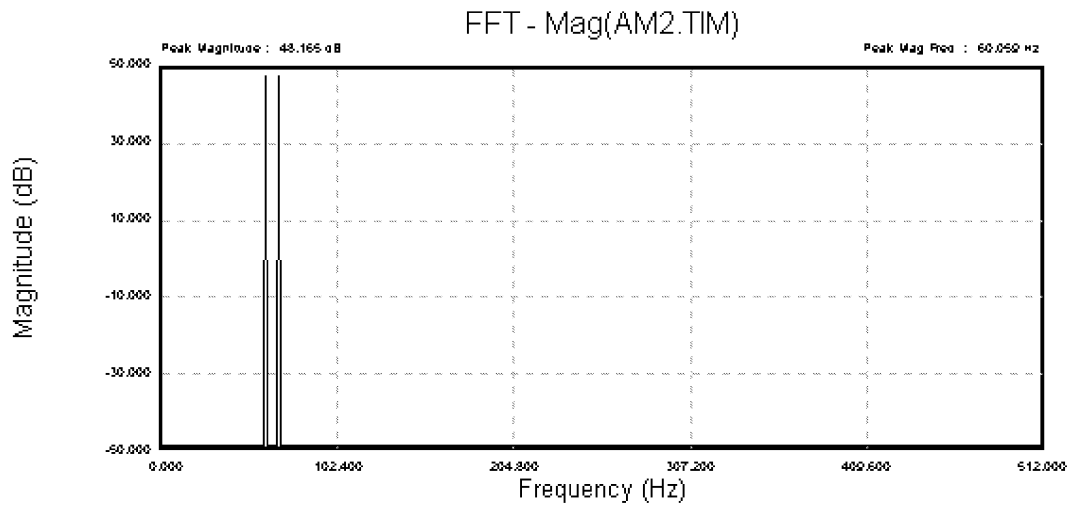
Figure 5. The FFT-Magnitude of the AM signal ( f_0 and f_c are located on the FFT-bin).
