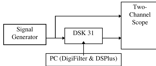
Figure 1. The laboratory set up for real-time filtering operation.
