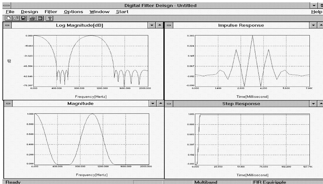
Figure 2. FIR multiband filter designed by using Park-McClellan method.
