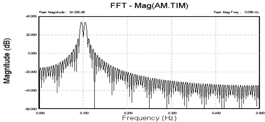
Figure 4. The FFT-Magnitude of the AM signal ( f_0 and f_c are not located on the FFT-bin).
