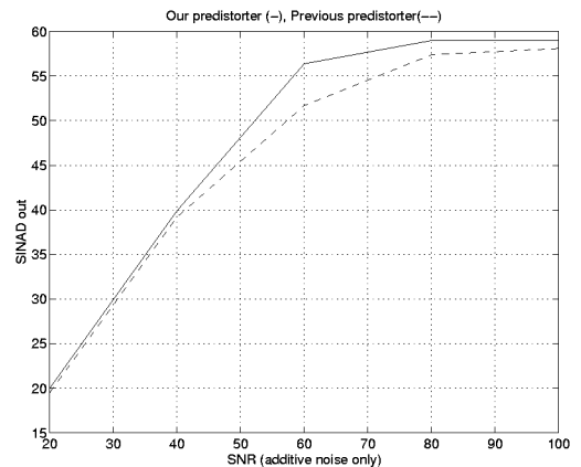
Figure 7: Simulation Results New(-)vs Old(- -)
