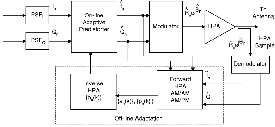
Figure 3: New Adaptive Predistorter
