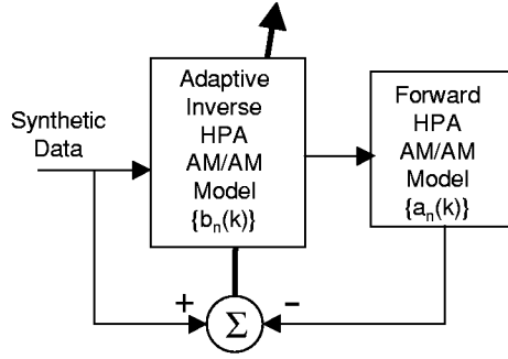
Figure 6: AM/AM Inverse Modeling
