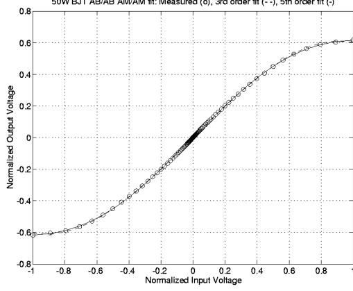
Figure 2: BJT class AB AM Char.
