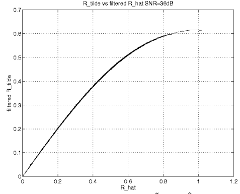
Figure 5: Filtered \tilde{R}_n vs \hat{R}_n
