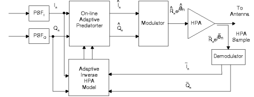
Figure 1: Prior Predistortion Methods
