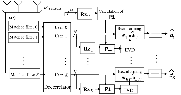
Figure 2. Proposed spatial-temporal detector.
