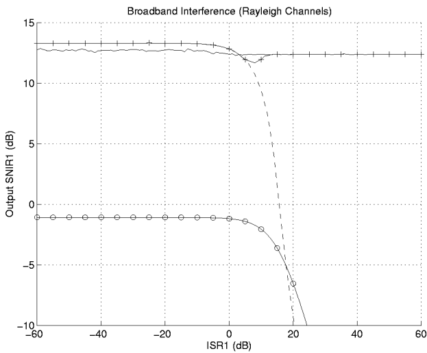
Figure 3. Output SNIR versus ISR for the 1st user. K=4 , I=1 . SNR1=-10dB, SNR2=-5dB, SNR3=0dB and SNR4=-5dB. Conventional receiver (-.-.). Choi's receiver [4] (- -). Proposed receiver (+). Proposed receiver with projection inhibited when the eigenvalue dispersion in matrix \mathbf{Rz}_0 is greater than 2 (+++).
