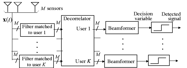
Figure 1. Choi's spatial-temporal detector [4].
