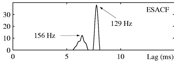
Figure 7: Result of pitch estimation on a signal consisting of vowels /a/ (129 Hz) and /i/ (156 Hz).
